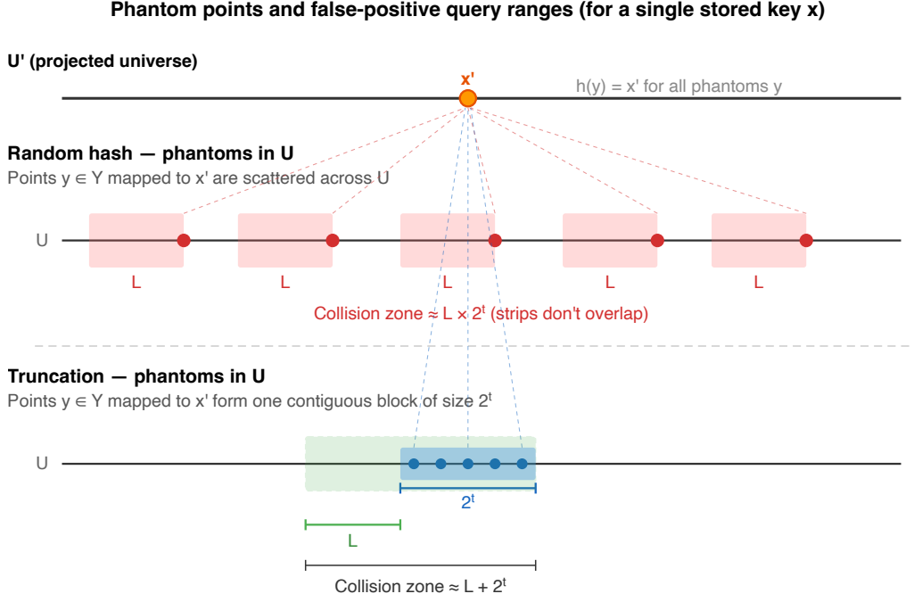
Figure 4.3: Phantom point distribution: random hash (SODA) scatters phantoms uniformly across U ; truncation concentrates them in a contiguous block adjacent to the key.
