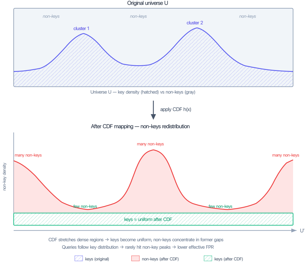
Figure 4.5: CDF redistribution. Top: original universe with non-uniform key density (uniform background + two clusters). After CDF mapping: keys become near-uniform, non-key density inverts — valleys where clusters were (low FPR), peaks where gaps were (high FPR, but queries rarely land there).
