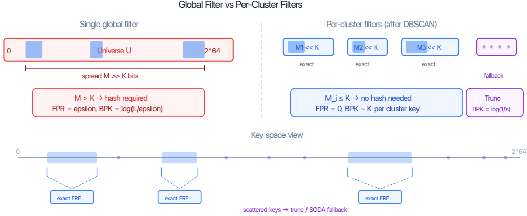
Figure 5.2: Global filter vs per-cluster exact filters. A single global universe forces hashing (nonzero FPR). Isolating each cluster into its own universe enables exact mode (FPR = 0) with fewer bits per key.
