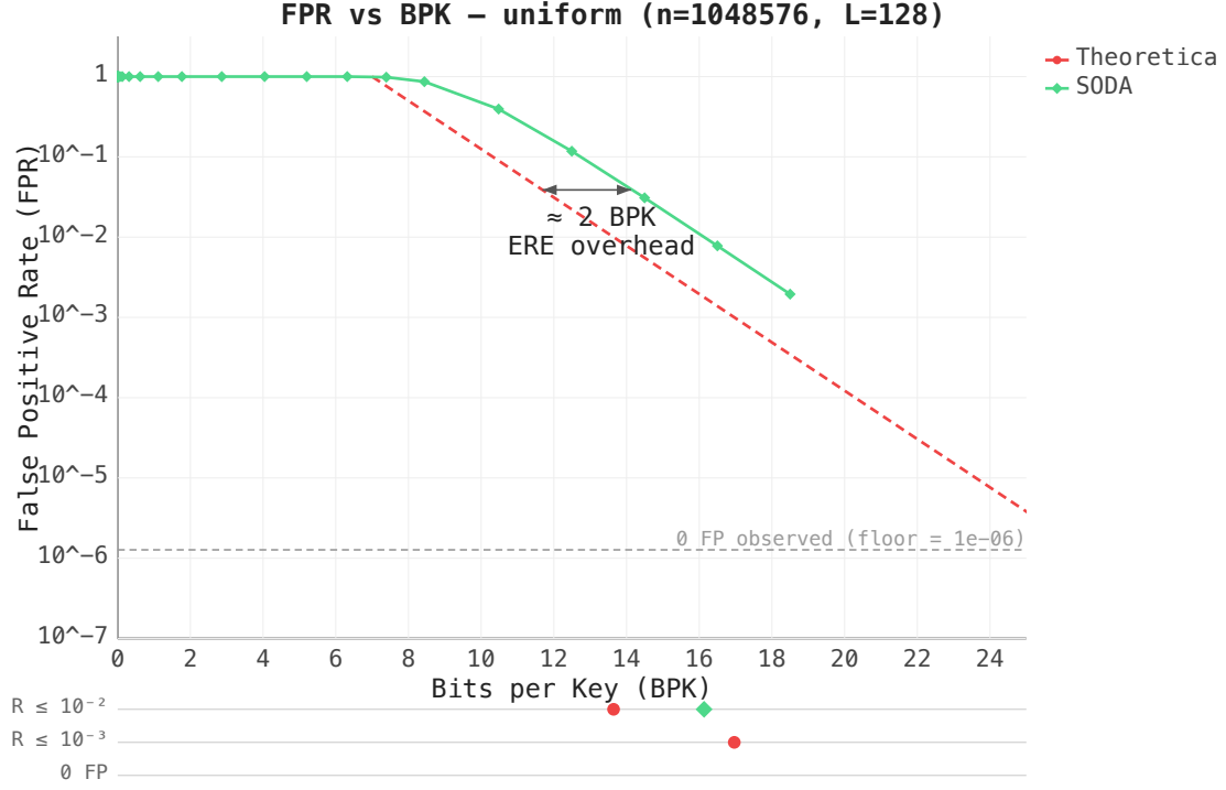
Figure 4.2: FPR vs BPK on uniform keys ( n = 2^{20} , \mathcal{L} = 128 ). SODA tracks the theoretical bound with \sim 2 BPK overhead from ERE metadata.
