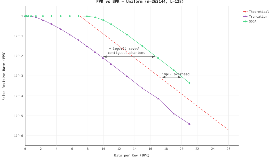
Figure 4.4: FPR vs BPK for truncation vs SODA on uniform keys ( n = 2^{18} , \mathcal{L} = 128 ). The SODA curve is shifted right by \approx \log_2(128) = 7 BPK — matching the theoretical prediction.
