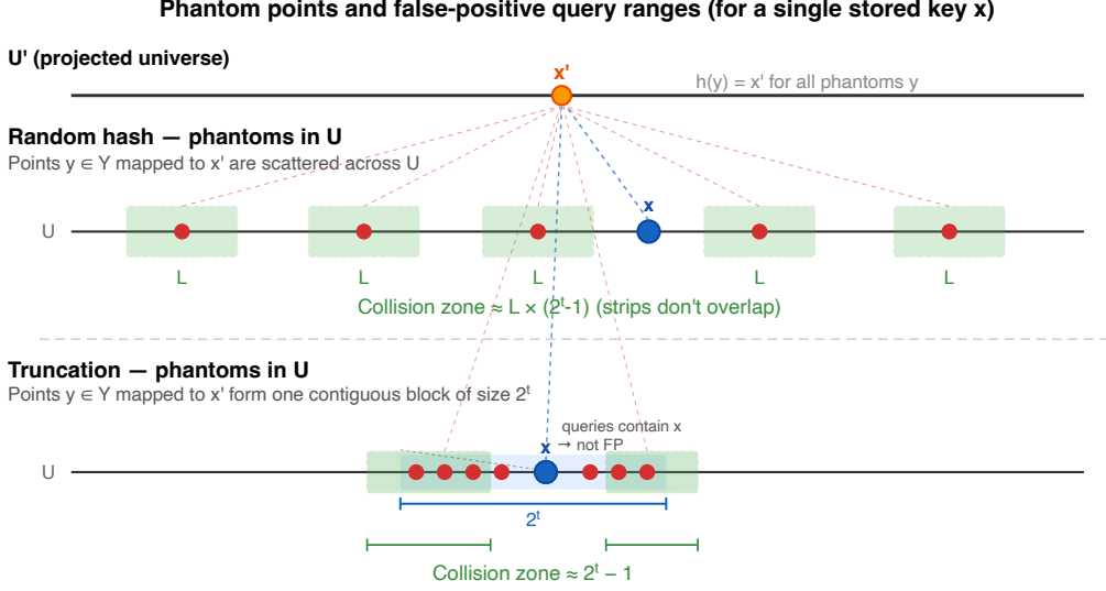
Figure 4.3: Phantom point distribution: random hash (SODA) scatters phantoms uniformly across U ; truncation concentrates them in a contiguous block adjacent to the key.
