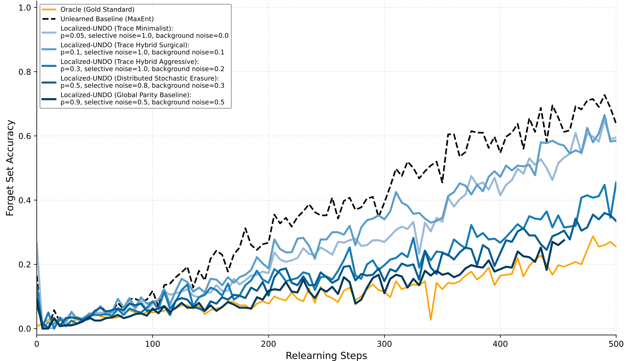
Relearning Attack Robustness (LR: 0.001)
