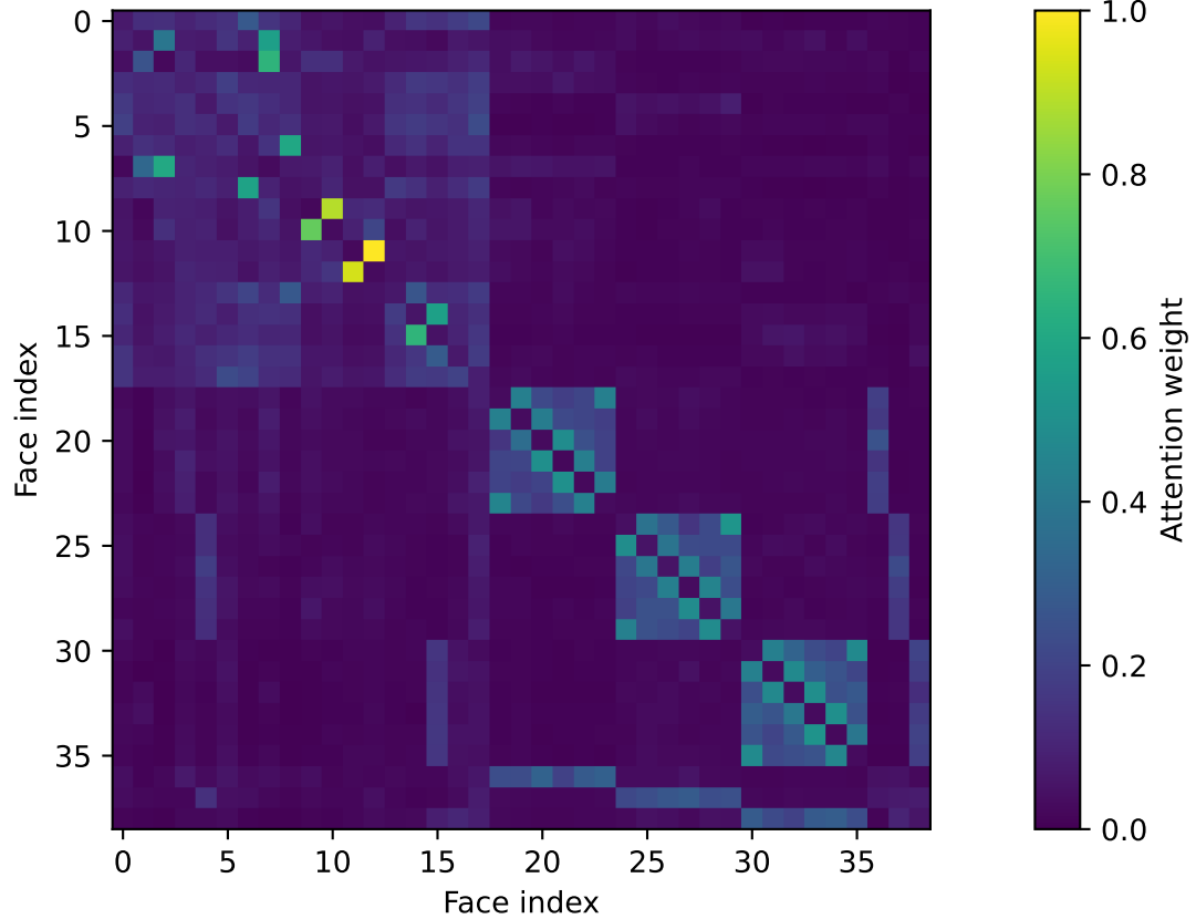
IAG-Transformer
