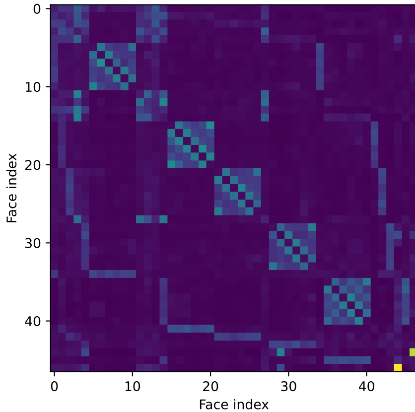
IAG-Transformer
