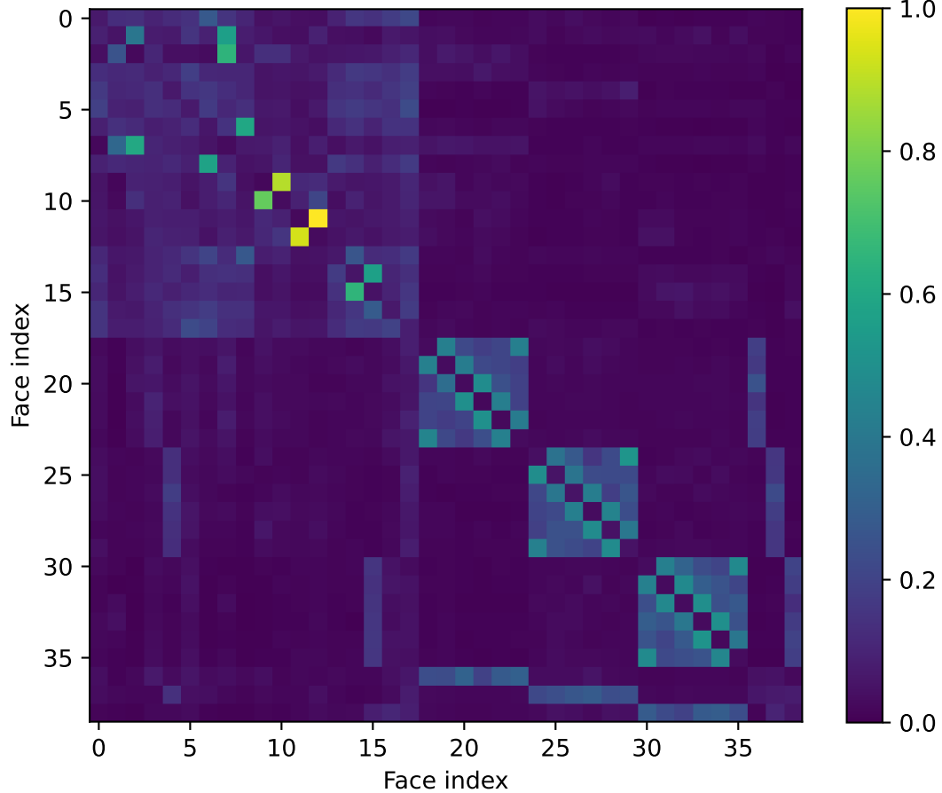
IAG-Transformer
