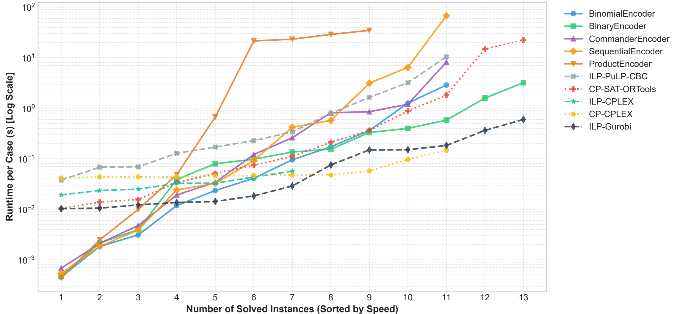
Cactus Plot: Runtime vs Solved Instances
