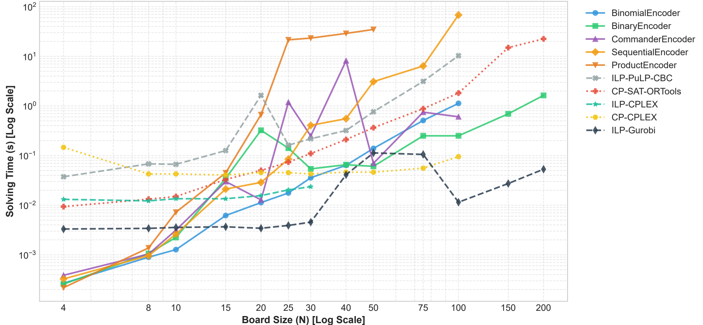
Solving Time Comparison Across Approaches (Log-Log)
