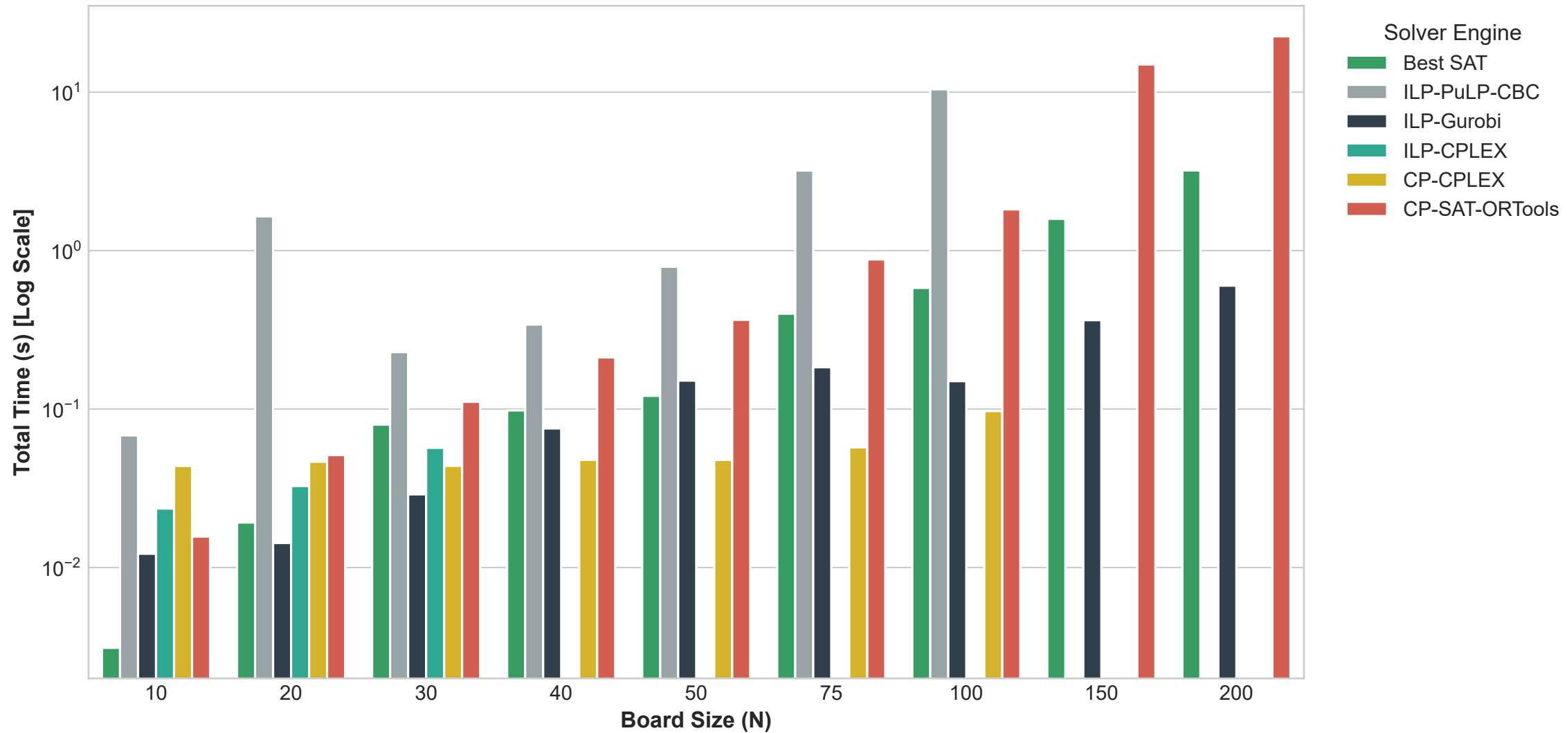
Benchmark: Best SAT vs Exact Methods
