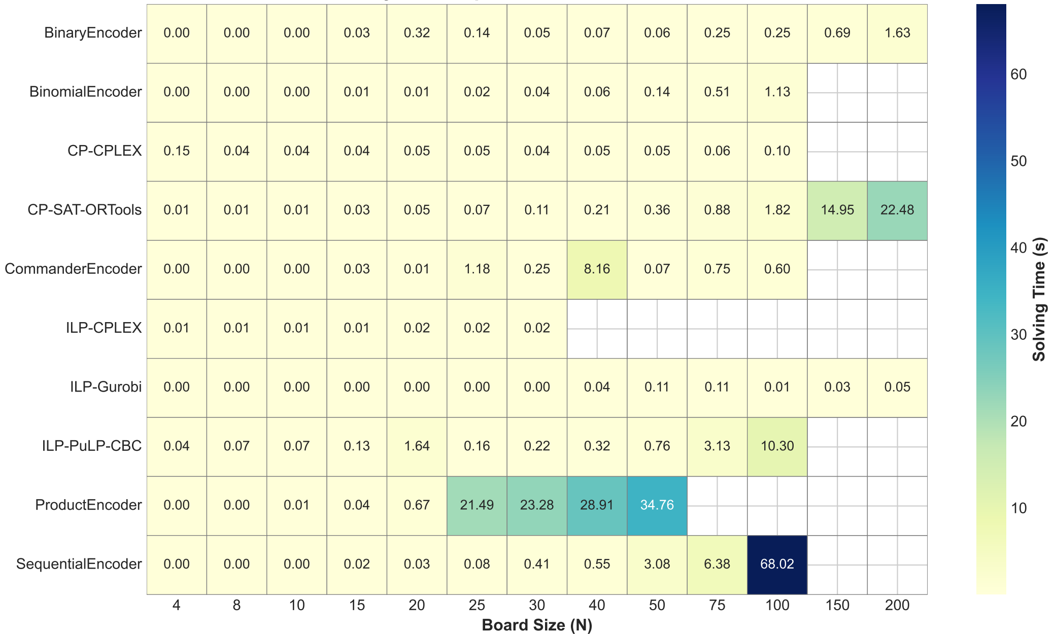
Scalability Heatmap: Performance Matrix across N
