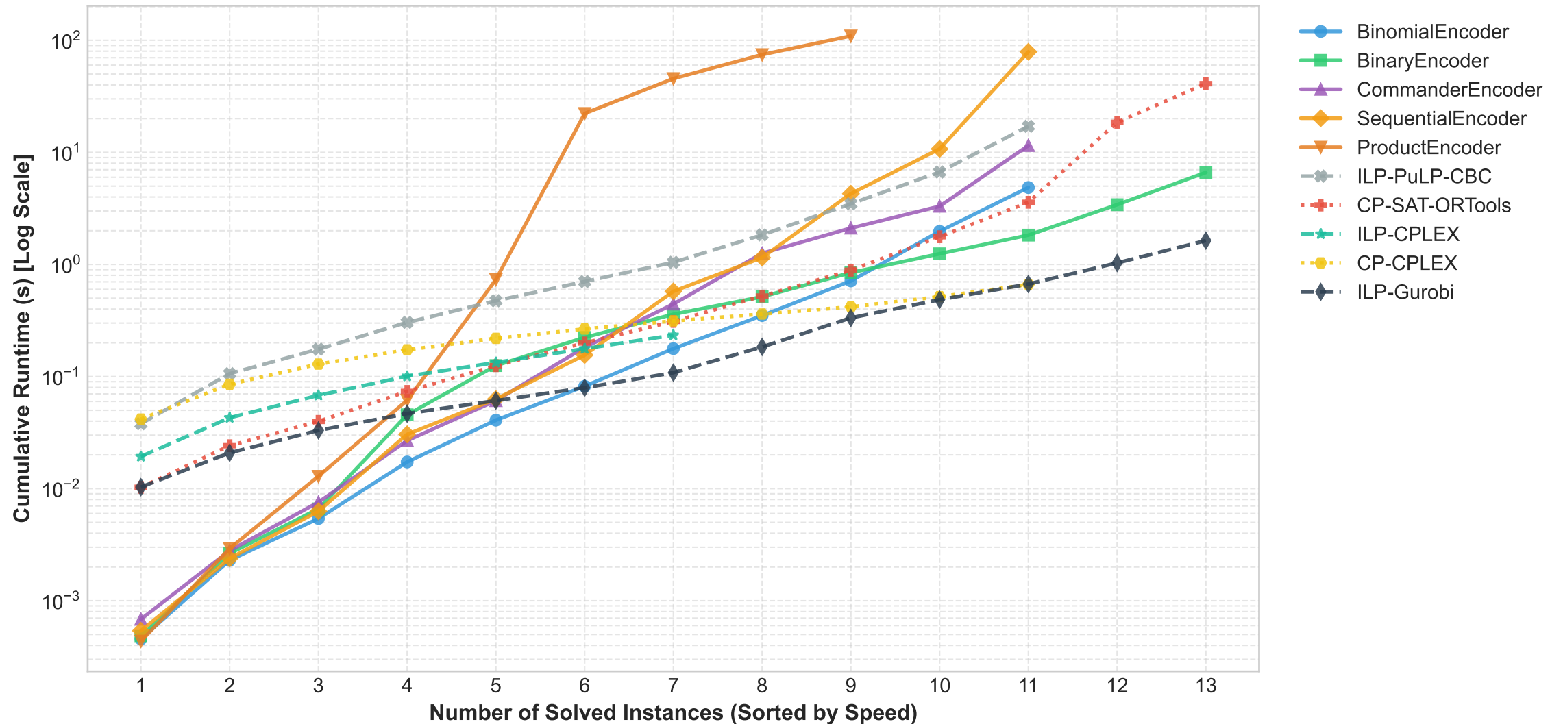
Cactus Plot: Cumulative Runtime vs Solved Instances
