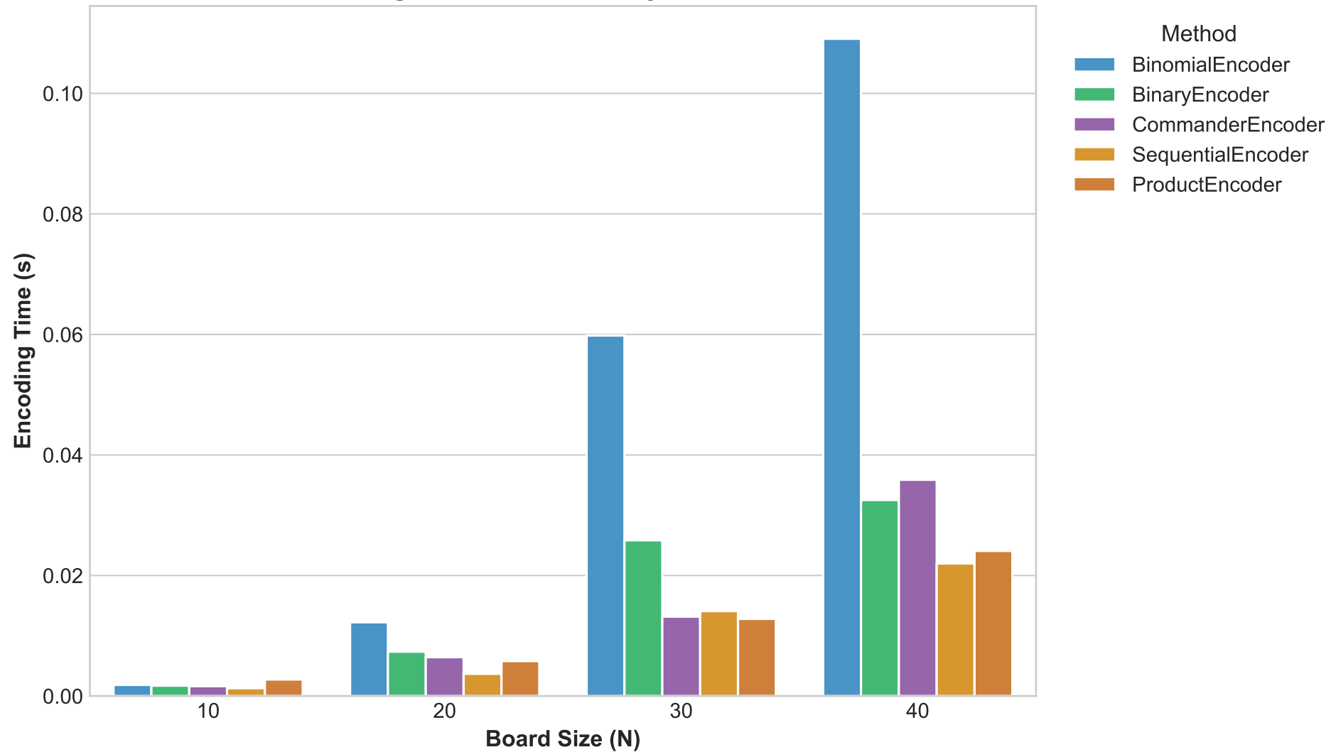
Encoding Time Overhead by SAT Encoder
