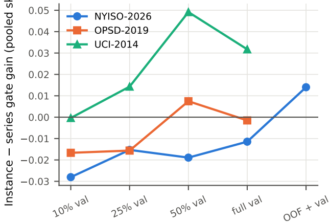
Estimation cost: gain of fine gates rises with data
