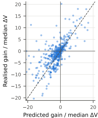
Unit axis: sign accuracy 0.89
