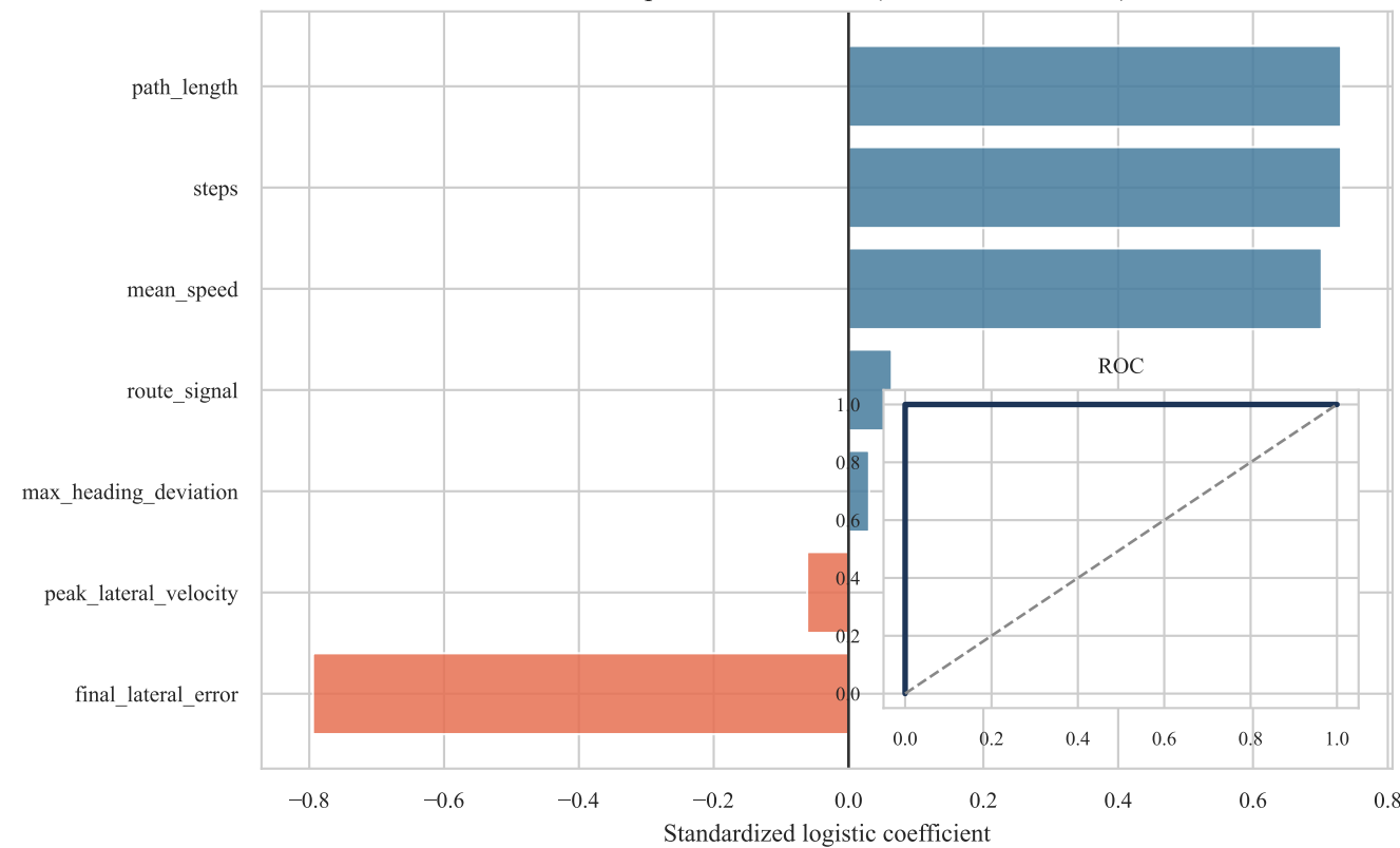
Outcome prediction drivers (ROC AUC = 1.000)
