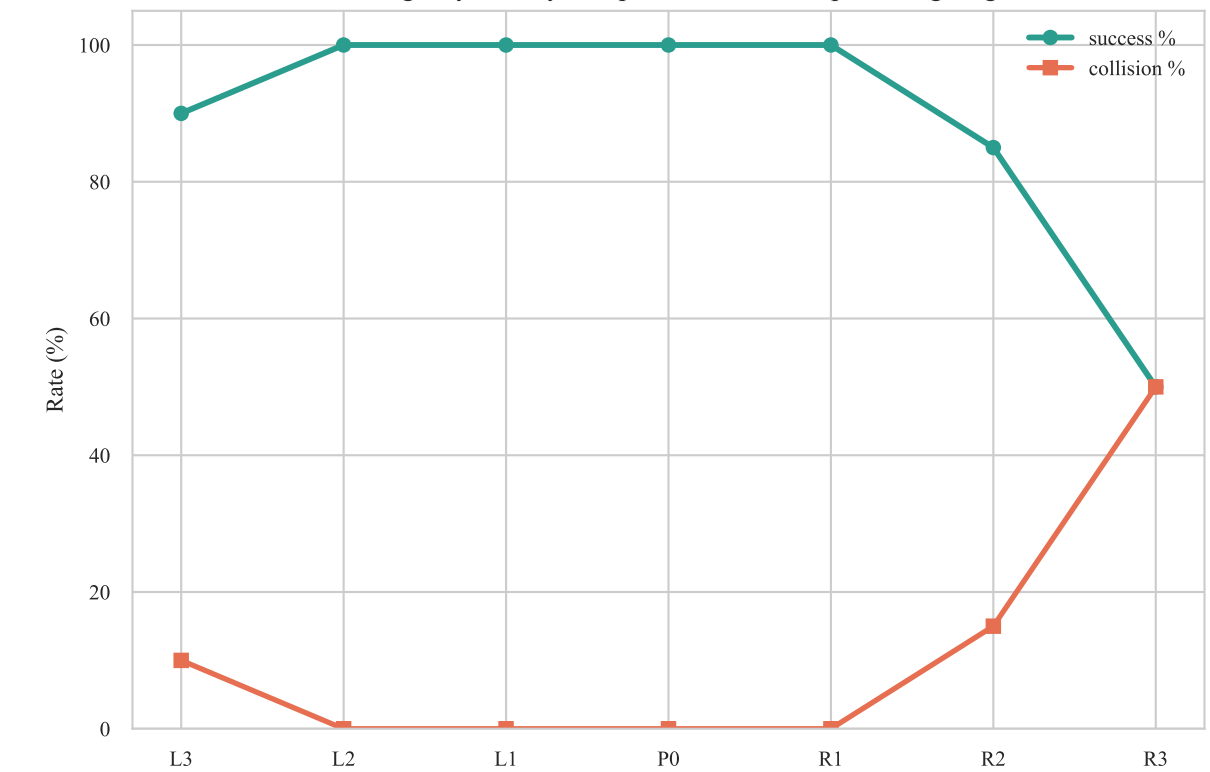
Perturbation tuning: asymmetry and performance collapse at high rightward force
