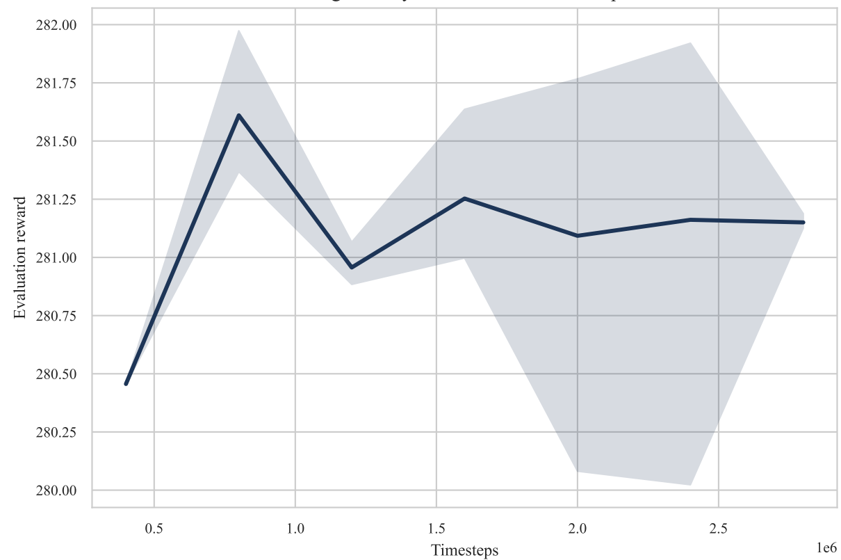
Perturbation tuning: asymmetry and performance collapse at high rightward force
