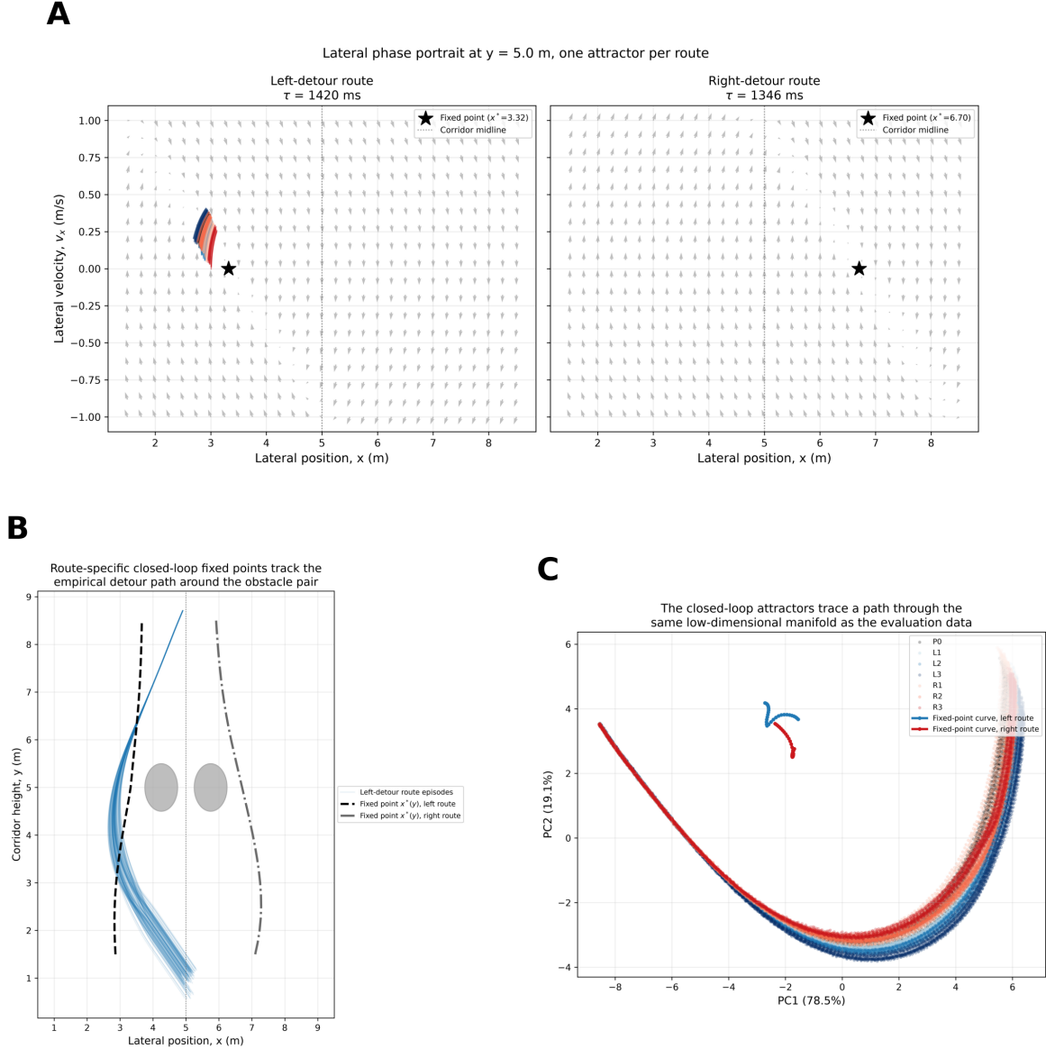
Figure 7: A closed-loop fixed-point analysis explains the location of the manifold and its clusters. (A) Lateral phase portrait at the corridor height where the perturbation is delivered ( y = 5.0 m), for the left- and right-detour routes. Grey arrows show the closed-loop vector field (policy and physics, perturbation off); coloured traces are real evaluation episodes passing through this band, coloured by perturbation condition as in Figure 3; the star marks the numerically solved fixed point. The right-route panel is a prediction, since the evaluation data sampled only the left route. (B) The fixed-point location x^*(y) computed across the full corridor height (dashed/dash-dot) tracks the empirical detour path (light blue) within a few centimetres at every height. (C) The same fixed-point curves projected into the PC1-PC2 space used for the clustering analysis in Figure 4, overlaid on the evaluation-condition scatter. The curves sit on the same manifold that the four phase-aligned clusters partition, at the location corresponding to steady, corrected cruising.
