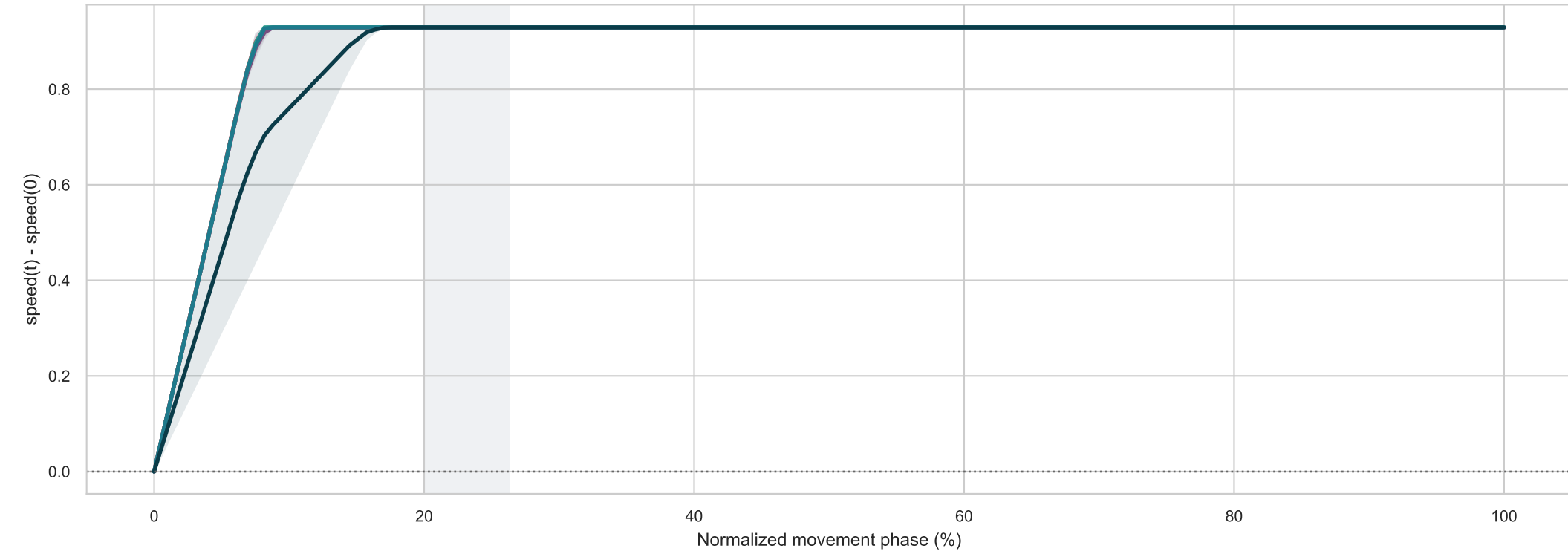
Speed modulation relative to movement onset reveals compensation intensity
