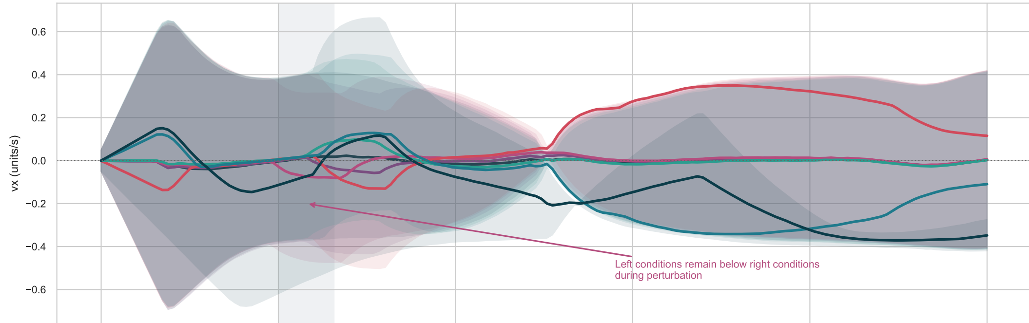
Speed modulation relative to movement onset reveals compensation intensity
