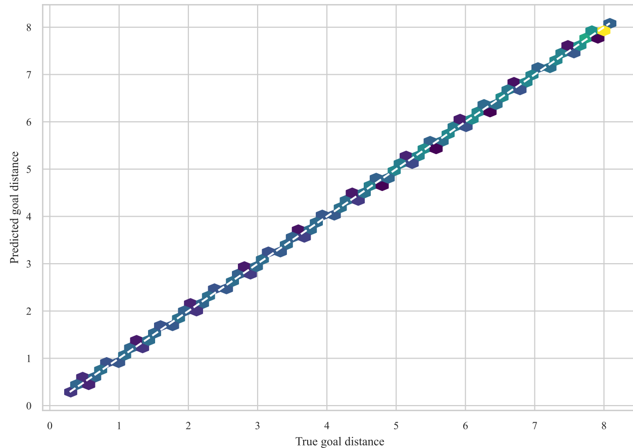
Goal-variable decoding from hidden state R2=1.000, MAE=0.006
