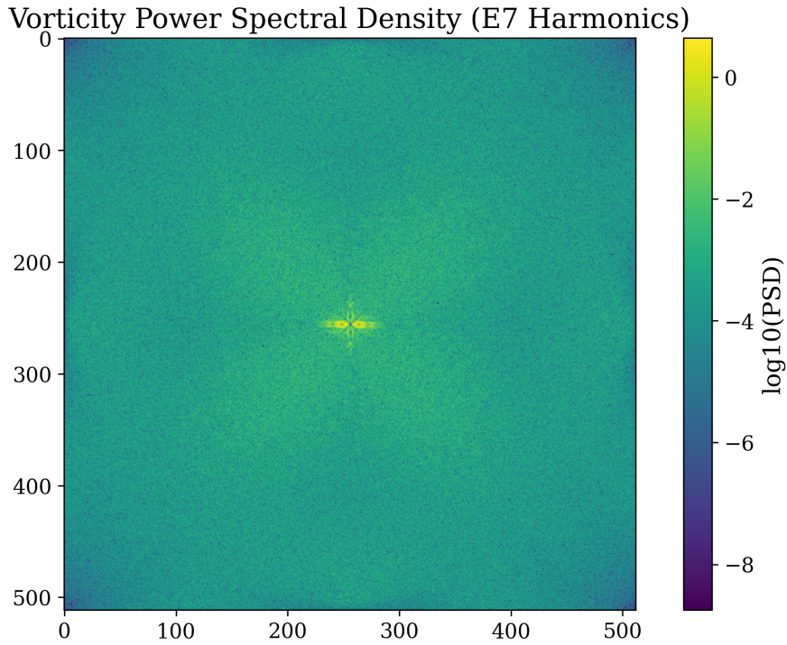
Figure 6.1: 2D PSD showing anisotropic spectral condensation. The energy is arrested at the Rhines scale k_\beta \approx 4 , forming the "Spine" of the physical regime.
