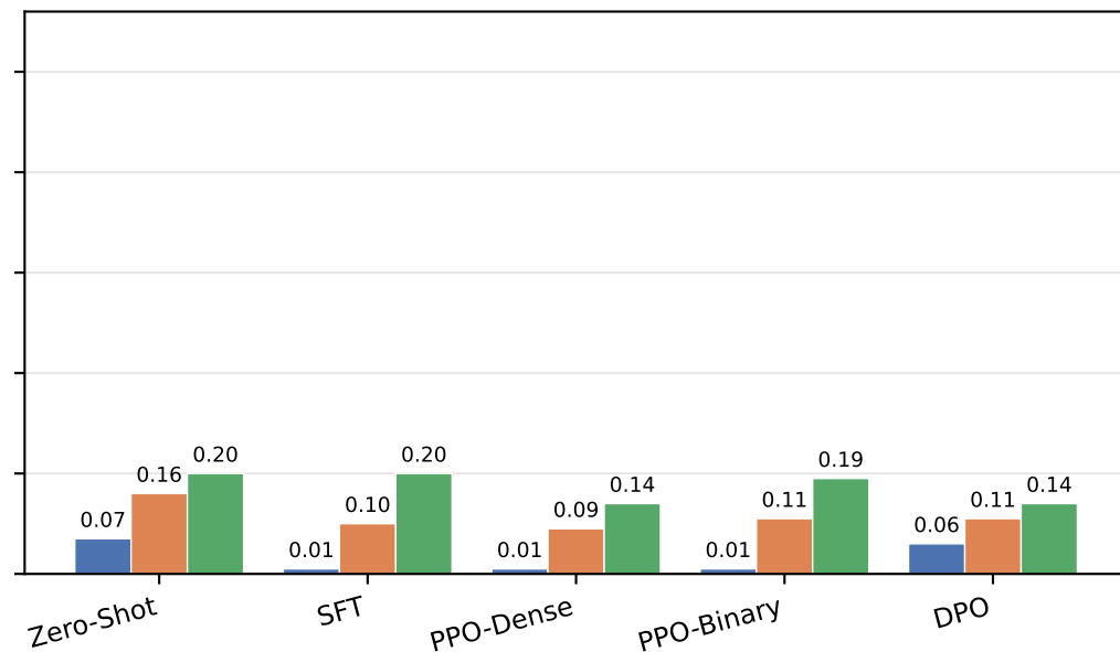
MBPP (first 100)
