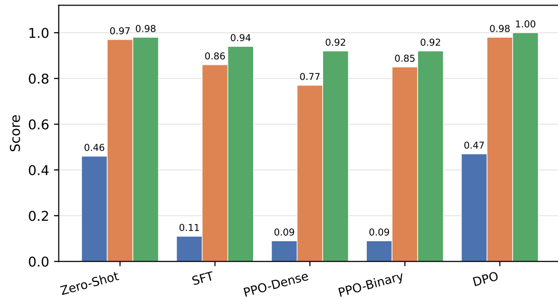
HumanEval (first 100)
