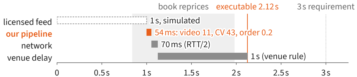
Figure 3. We can trade inside 3 s. Stage means of 24 traces: own footage over WebRTC into the CV engine on a laptop (on an L4 GPU: 4.6 ms; WebRTC video leg alone 4–8 ms), a simulated 1 s feed, the measured network and the 1 s venue hold; order built, not sent. Shaded: when the book reprices.
