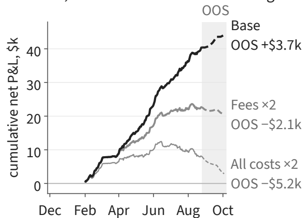
Figure 1. The edge exists at the fast tier's fills. (a) Monthly net 30 s markout (copying 3 s later: held to resolution). (b) v2 net P&L. Filled / solid = IS, hollow / dashed = burned OOS.
