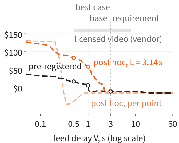
Figure 2. Each second of feed delay costs the edge. CV strategy, (a) IS and (b) burned OOS, by stamp-lag reading; dots: the scenarios of Table 1B; grey bar: licensed video (vendor-stated). Simulated: assumed feed latency (licensed feed not purchased); parameters measured.
