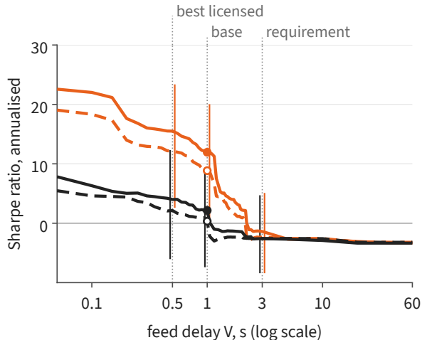
b At 1 s, Sharpe hinges on the stamp lag
