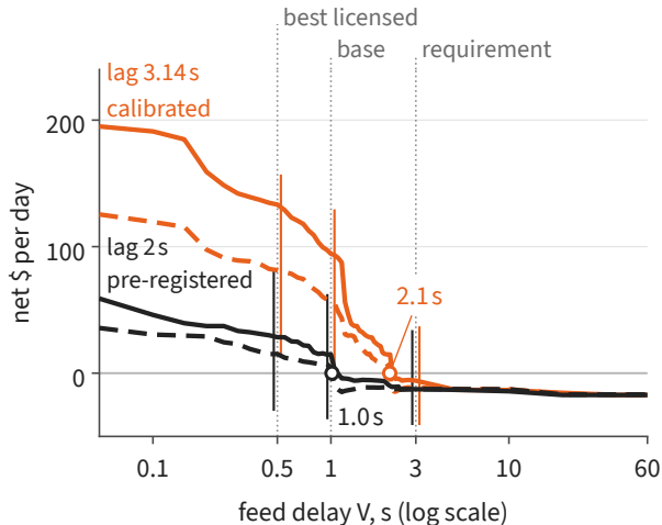
a Profit hits zero at 1.0–2.1 s of delay
