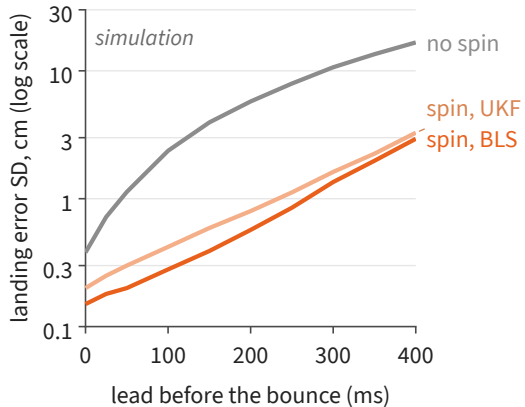
a Spin-aware fit cuts error 10× at 200 ms
