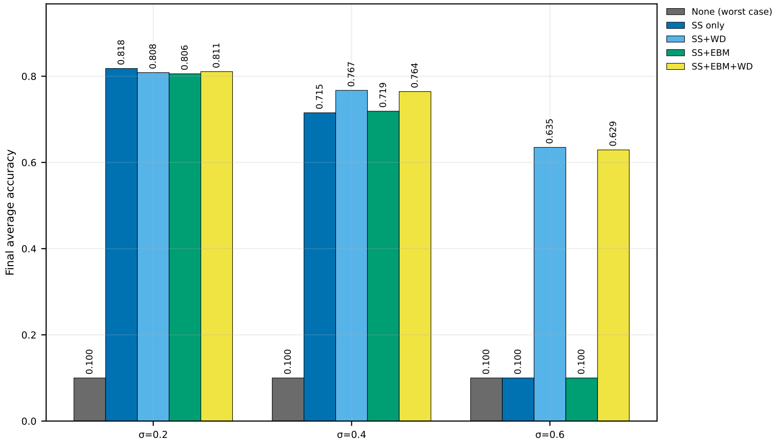
Ablation Groups (Byzantine Attack) | CIFAR-10 | CART | seed=2026 (IID)
