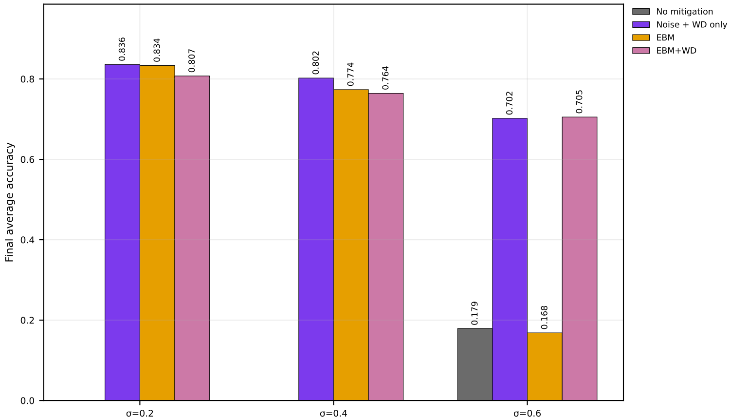
Ablation Groups (Channel Noise) | CIFAR-10 | MERGED | seed=2025 (IID)
