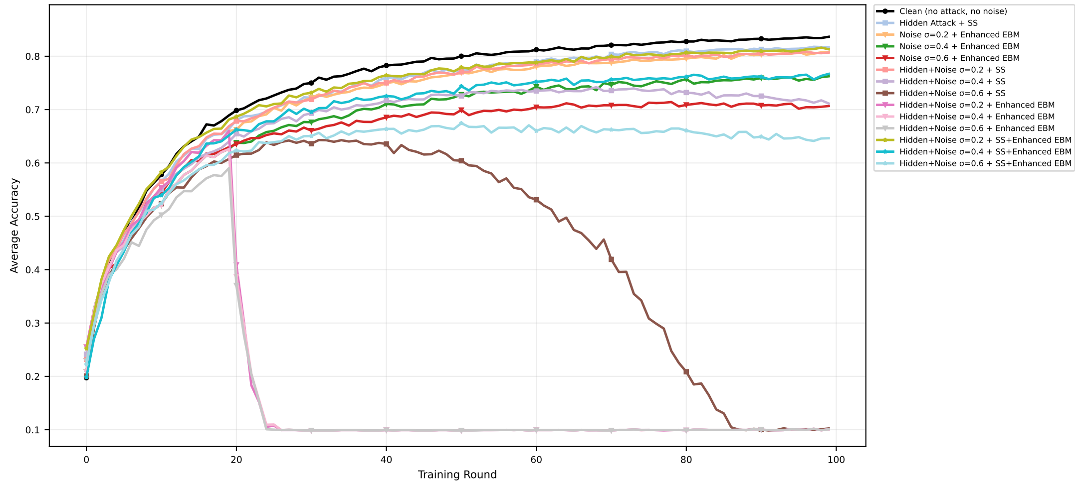
Zoomed Accuracy | CIFAR-10 | MERGED | seed=2026 (IID)
