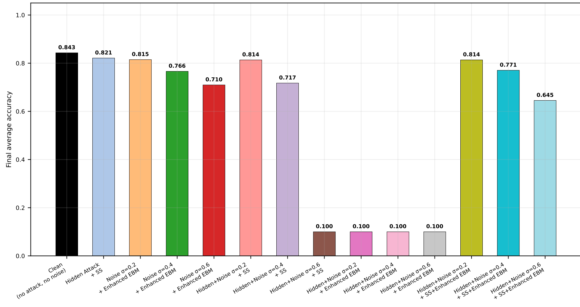
Final Accuracy | CIFAR-10 | MERGED | seed=2026 (IID)
