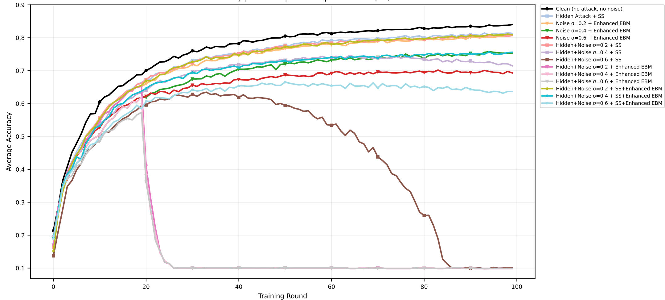
Zoomed Accuracy | CIFAR-10 | MERGED | seed=2028 (IID)
