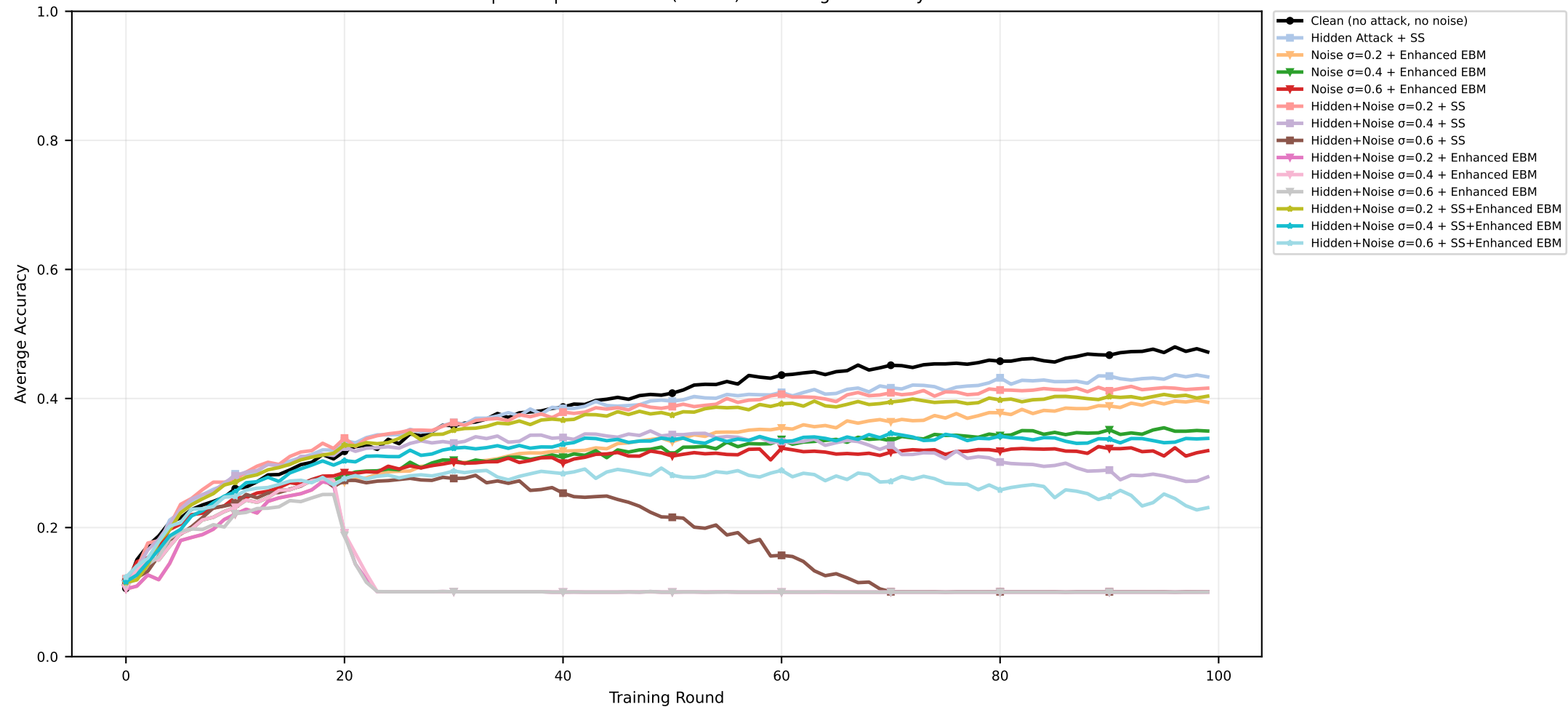
CIFAR-10 | CART | seed=2028 (nonIID) — Average Accuracy
