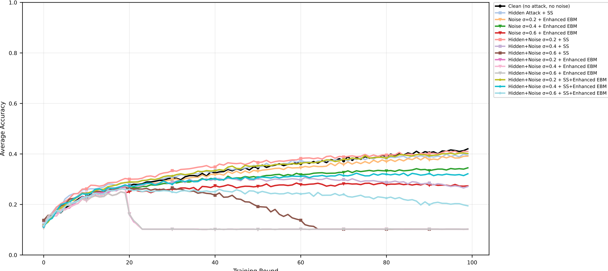
CIFAR-10 | MERGED | seed=2025 (nonIID) — Average Accuracy
