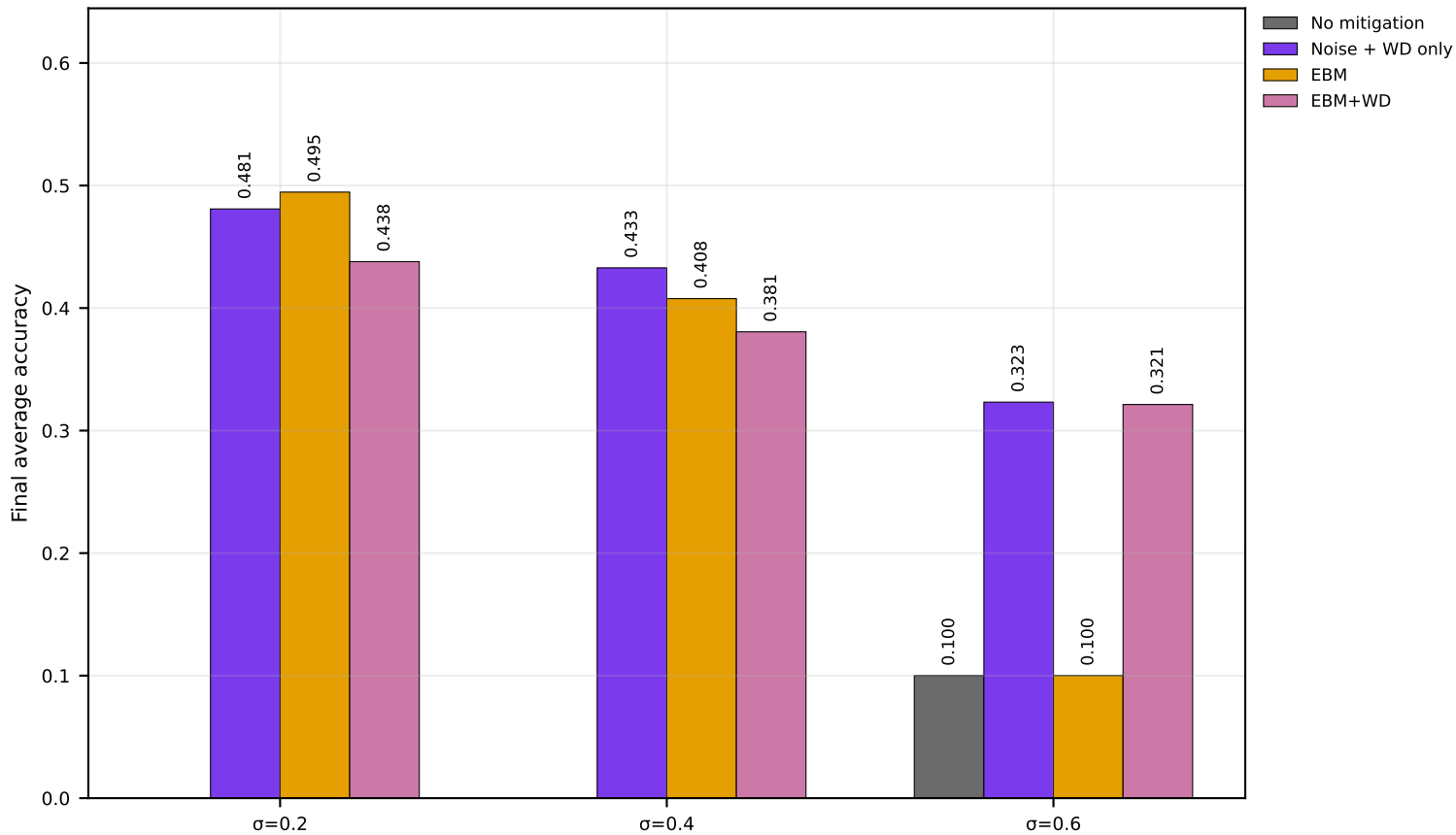
Ablation Groups (Channel Noise) | CIFAR-10 | MERGED | seed=2026 (nonIID)
