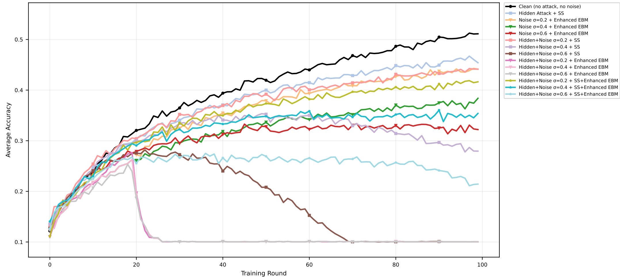
Zoomed Accuracy | CIFAR-10 | MERGED | seed=2026 (nonIID)
