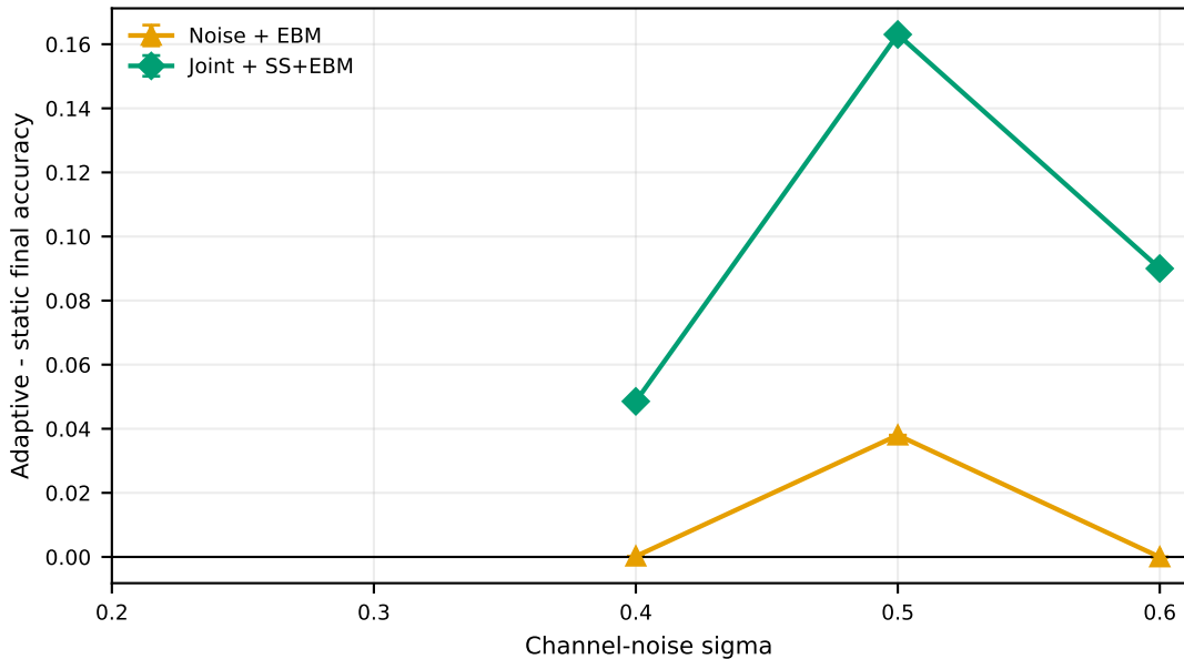
Paired adaptive EBM effect: MERGED (nonIID)
