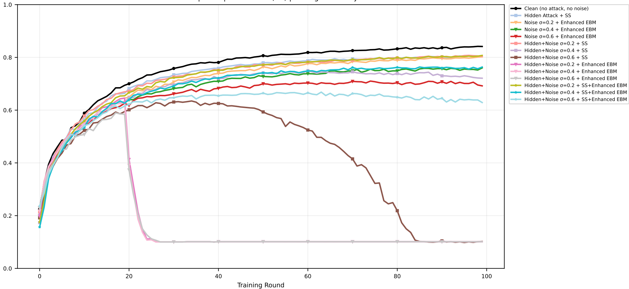
CIFAR-10 | CART | seed=2025 (IID) | Average Accuracy
