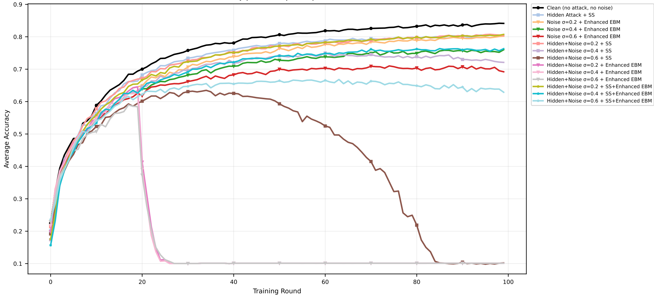
Zoomed Accuracy | CIFAR-10 | CART | seed=2025 (IID)
