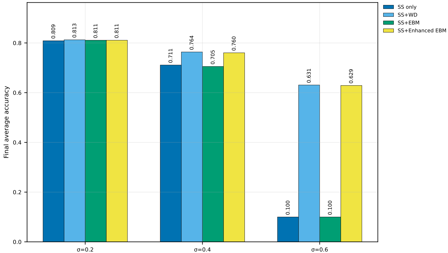
Ablation Groups (Byzantine Attack) | CIFAR-10 | CART | seed=2027 (IID)
