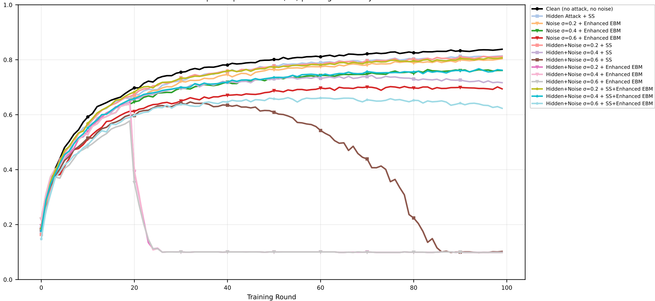
CIFAR-10 | CART | seed=2028 (IID) | Average Accuracy
