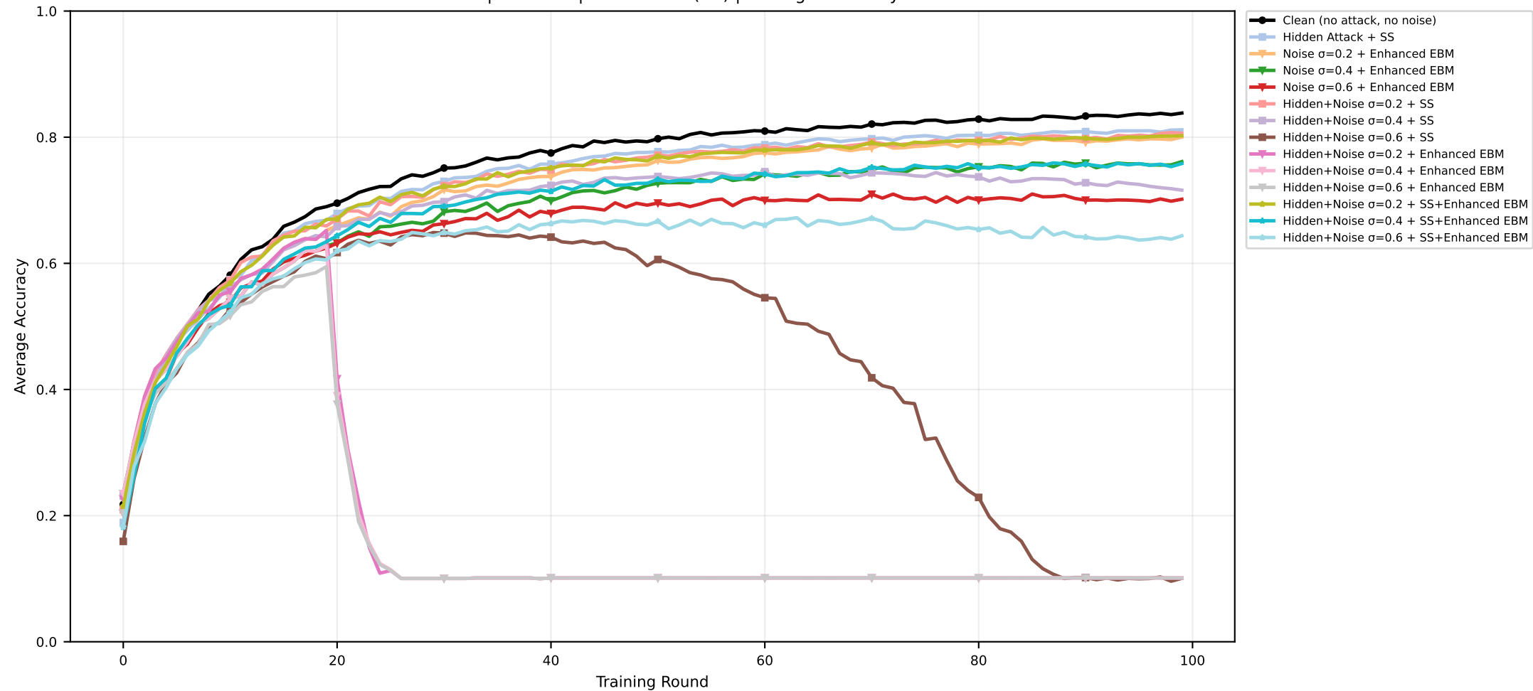
CIFAR-10 | MERGED | seed=2025 (IID) | Average Accuracy
