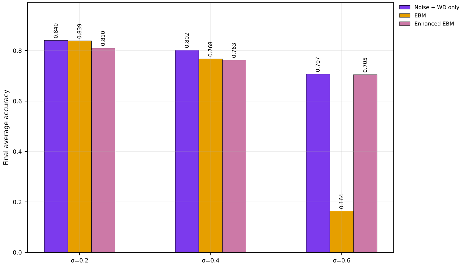
Ablation Groups (Channel Noise) | CIFAR-10 | MERGED | seed=2027 (IID)
