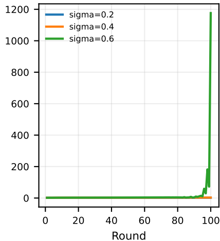
Combined pre-clip norm
