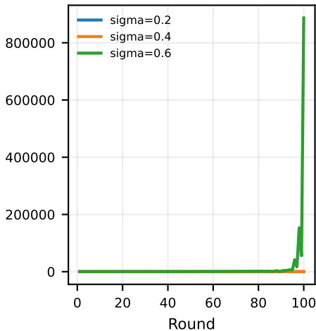
EBM regularizer gradient norm
