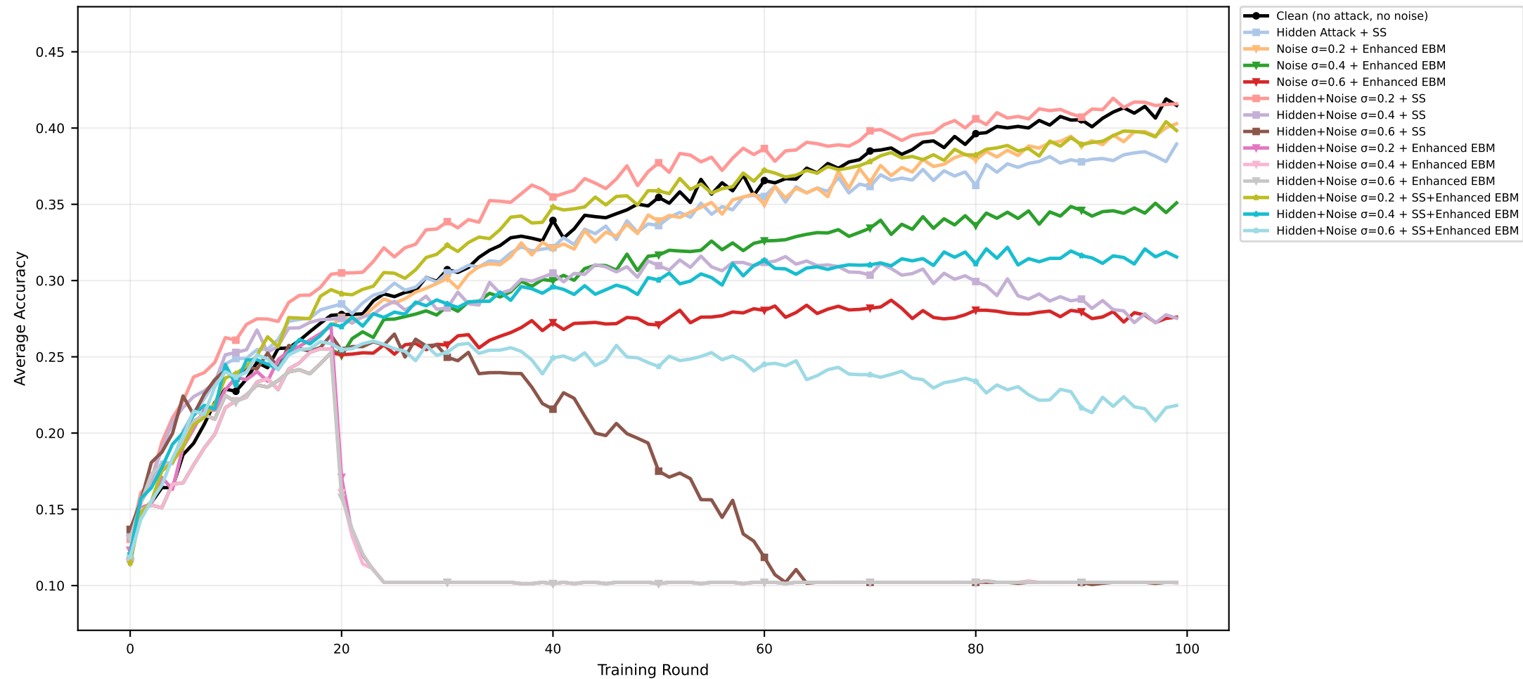
Zoomed Accuracy | CIFAR-10 | CART | seed=2025 (nonIID)
