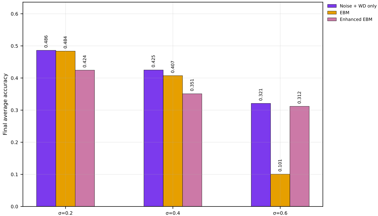
Ablation Groups (Channel Noise) | CIFAR-10 | CART | seed=2027 (nonIID)
