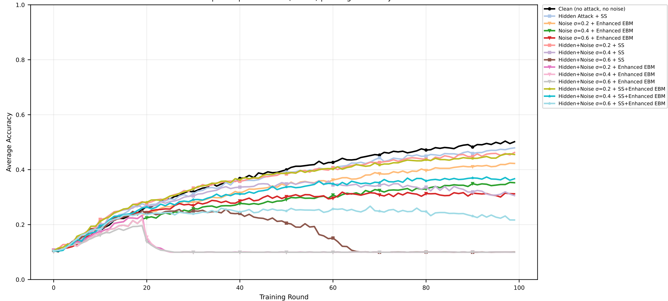
CIFAR-10 | CART | seed=2027 (nonIID) | Average Accuracy
