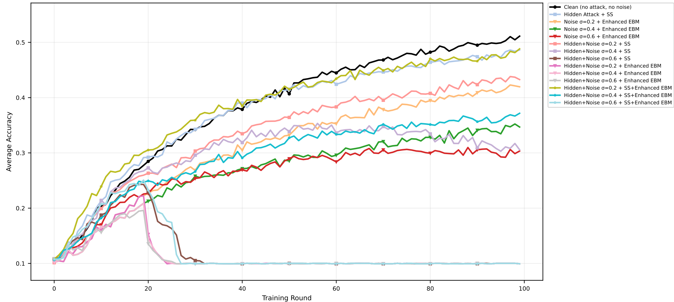
Zoomed Accuracy | CIFAR-10 | MERGED | seed=2027 (nonIID)
