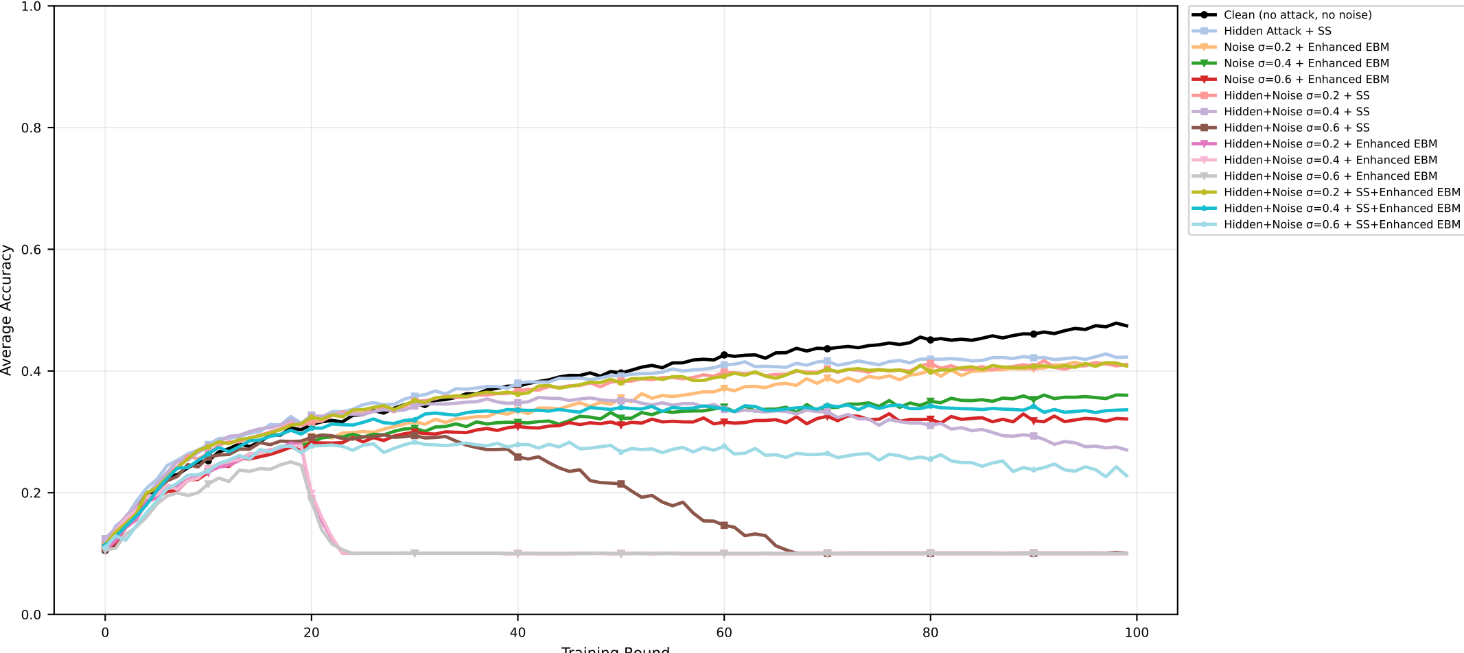
CIFAR-10 | MERGED | seed=2028 (nonIID) | Average Accuracy
