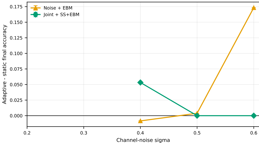
Paired adaptive EBM effect: CART (nonIID)
