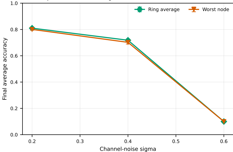
Joint SS+EBM average versus worst node: CART (IID)
