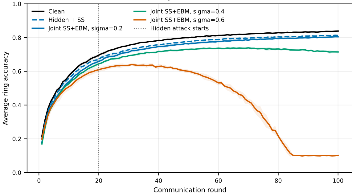
Learning curves: CART (IID)
