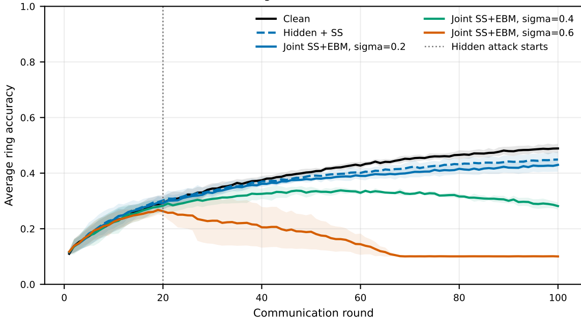
Learning curves: CART (nonIID)
