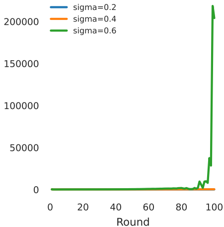
EBM regularizer gradient norm
